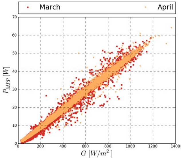
Figure 25: Power output of an a-Si module versus global in plane irradiance for two month of data
